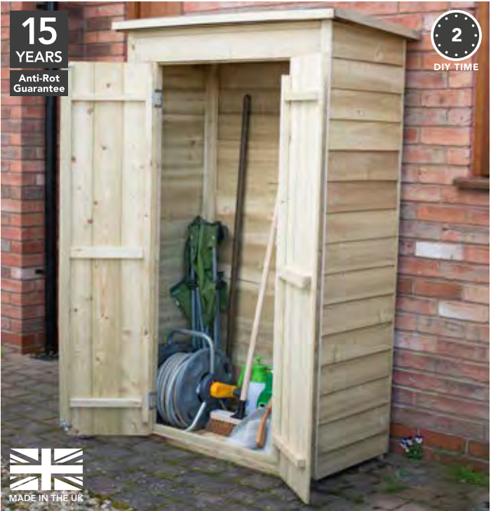
PENT TALL GARDEN STORE 178(h) x 108(w) x 55(d)cm HD OPPTGS(HD) IN OPPTGSIN
